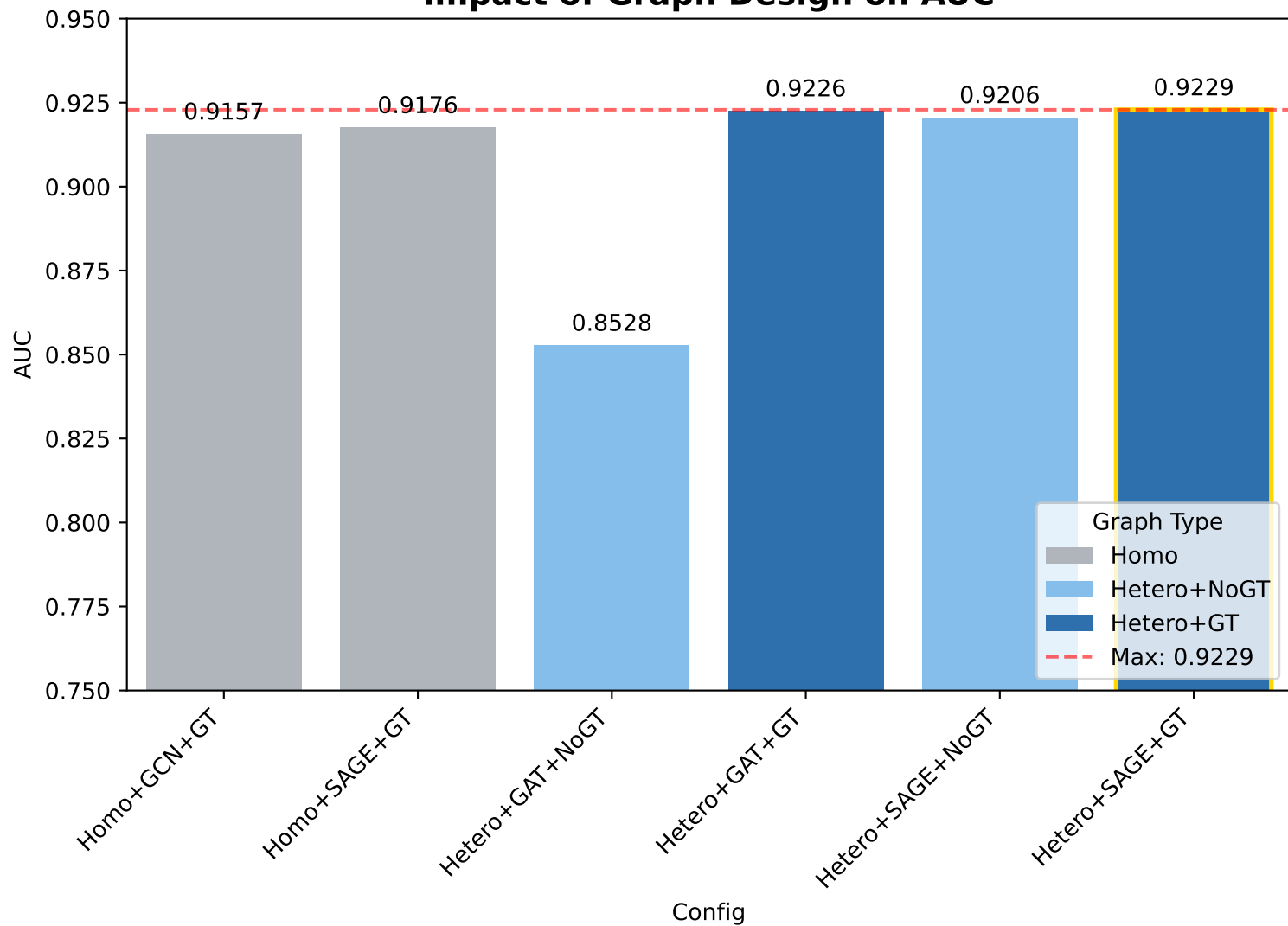
Impact of Graph Design on AUC
